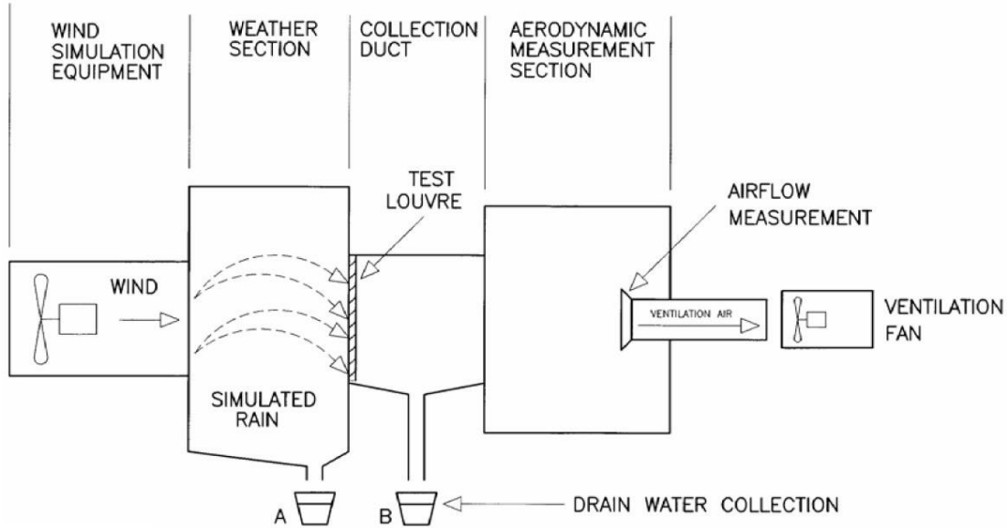
Figure 1: Diagram of Rain Penetration Test Set Up
